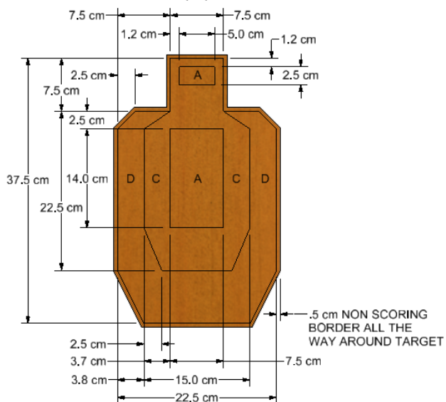
Half USPSA Target (cm)
