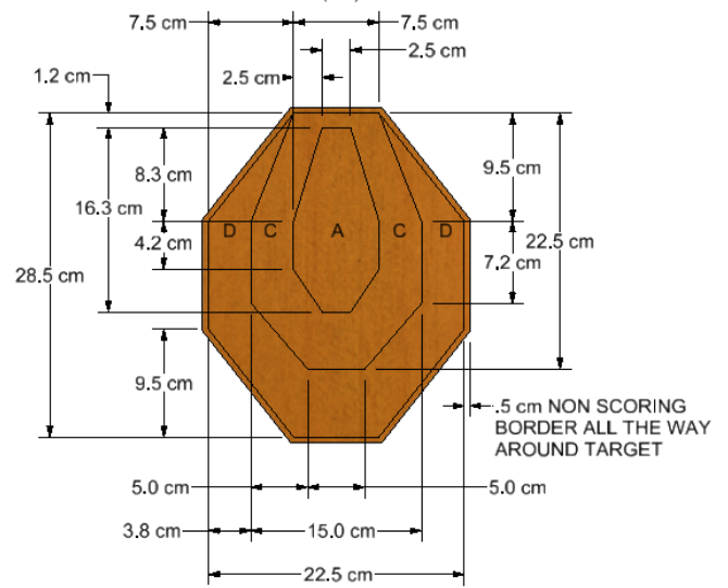
Half IPSC Target (cm)
