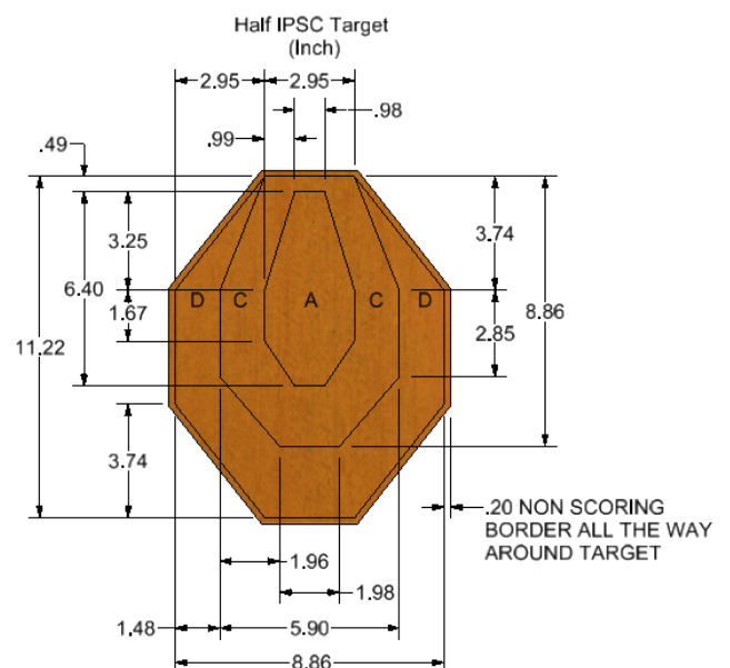
Half-size IPSC Target
